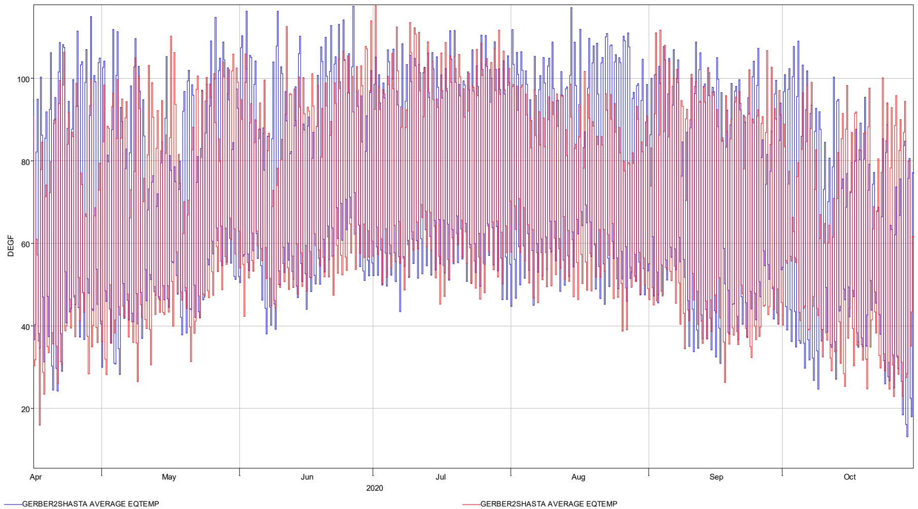
Figure 15. WY 2020 comparison of calculated equilibrium temperature (blue) to the forecasted equilibrium temperature used in a forecast run made on April 15 (red) at a 6-hourly time scale
