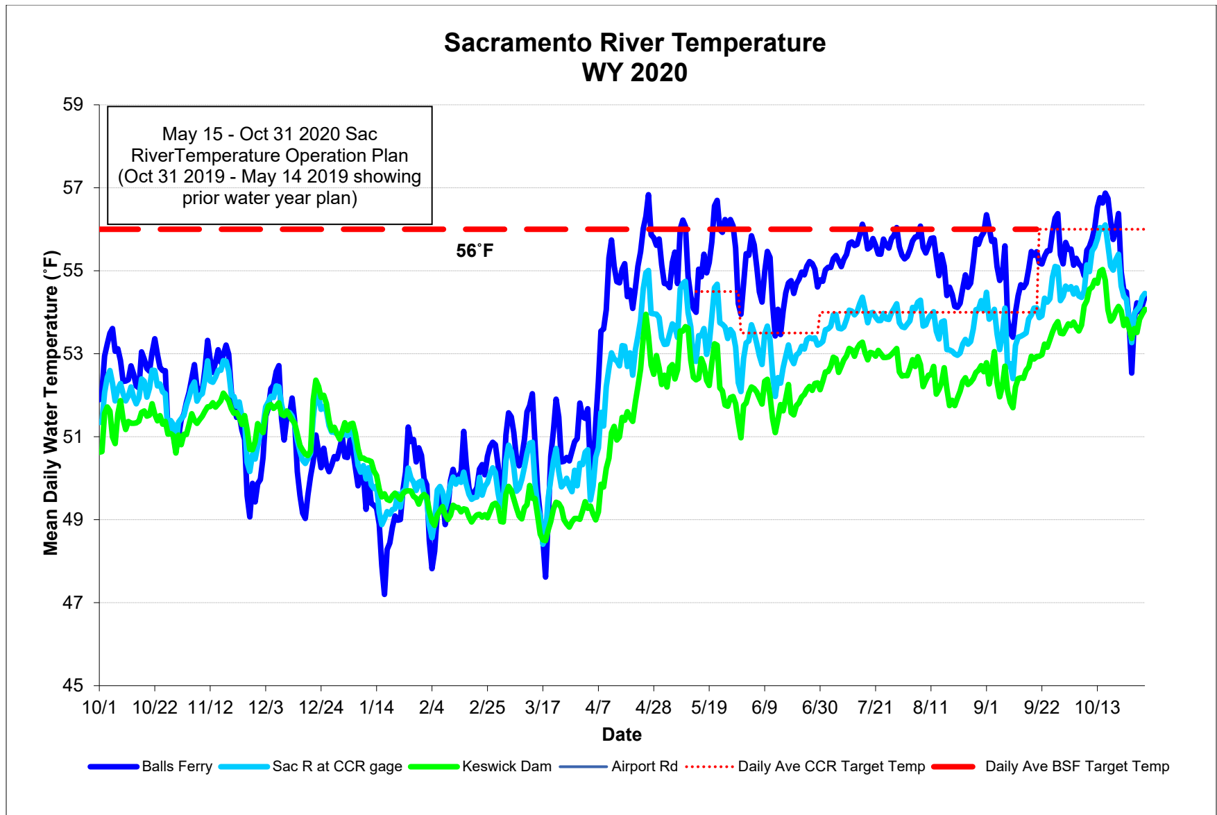
Figure 12. Summary of Upper Sacramento River Daily Mean Water Temperature in WY 2020.
