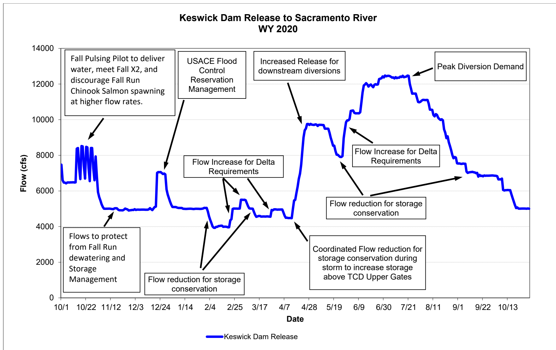
Figure 7. Sacramento River Releases from 10/1/2019 - 10/31/2020 with major events highlighted
