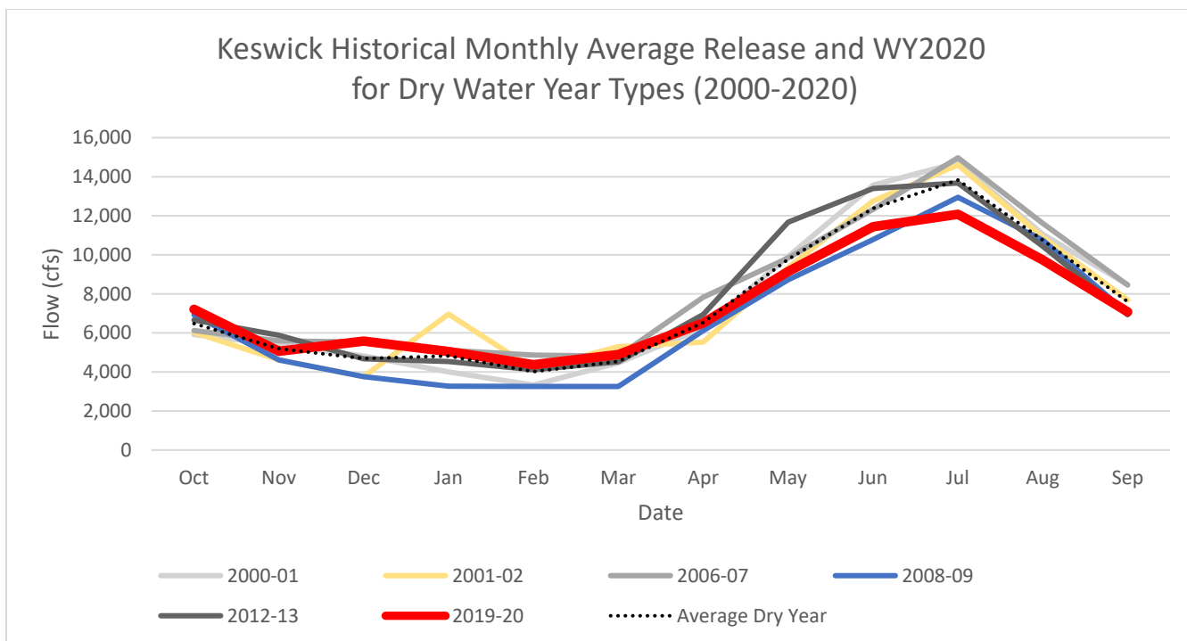
Figure 9. Keswick Historical Monthly Average Releases and WY2020 for Dry Water Year Types (2000-2020).
