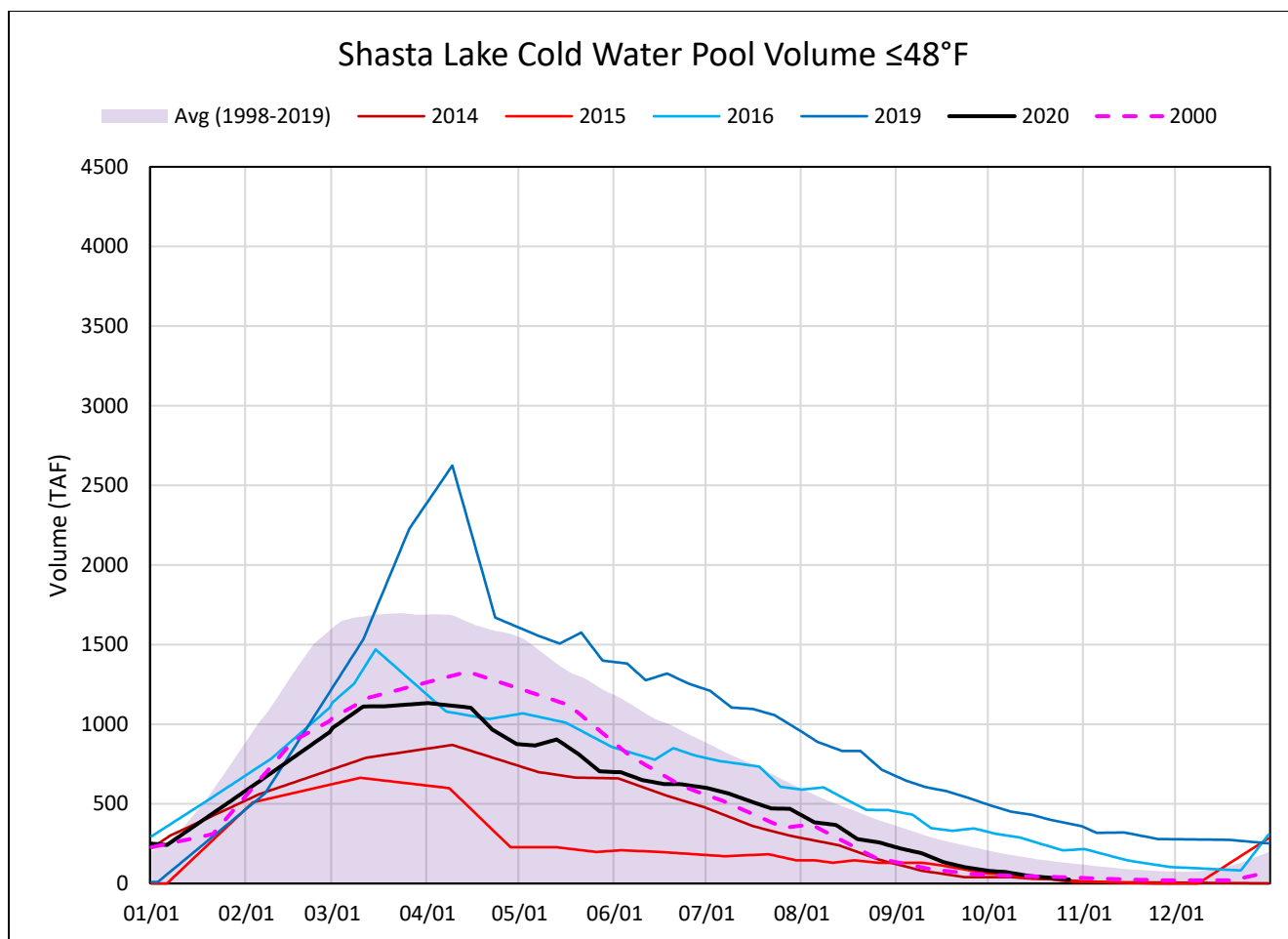
Figure 10. Shasta Lake cold water pool volume less than 48°F.
