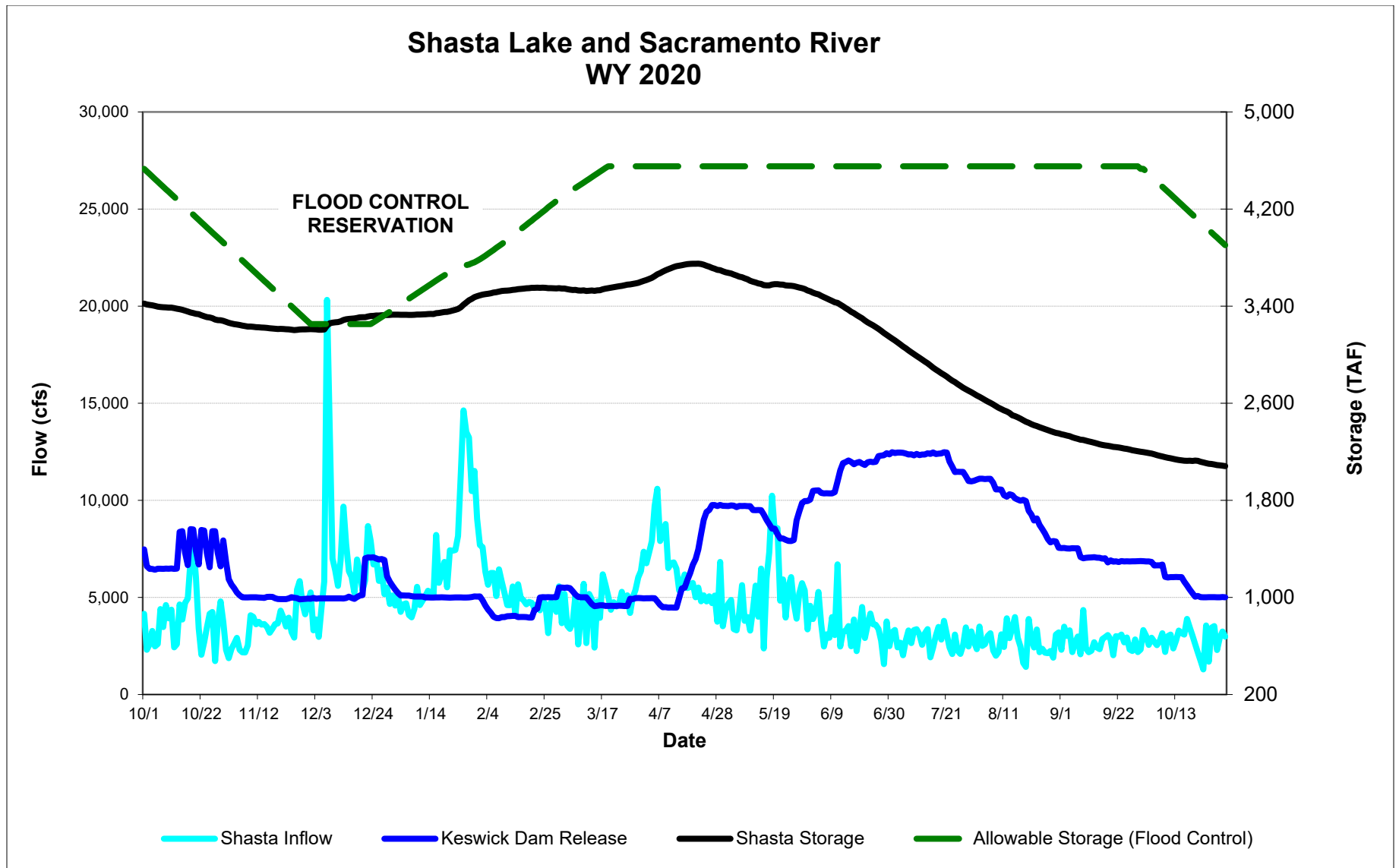
Figure 6. Shasta Lake Storage (black line), Allowable Storage for Flood Control (green line), Keswick Dam Release (dark blue line), and Shasta Inflow (light blue line) for 10/1/2019 - 10/31/2020.
